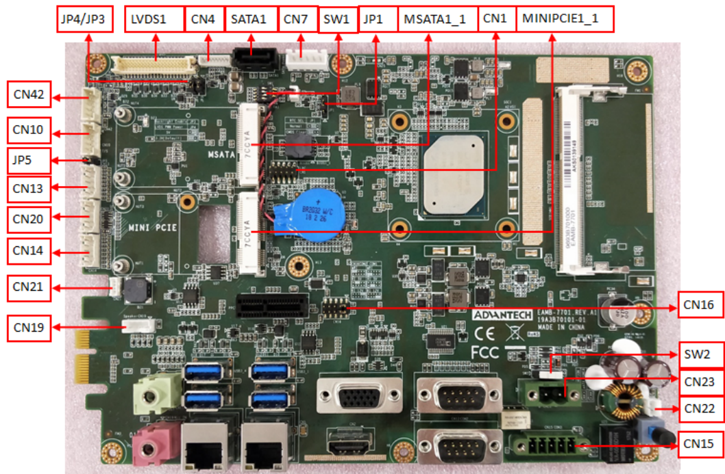
Motherboard layout diagram
