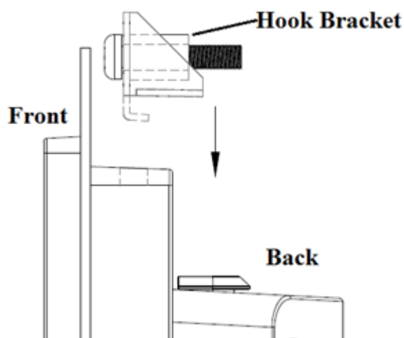
Hook brackets for panel mounting
