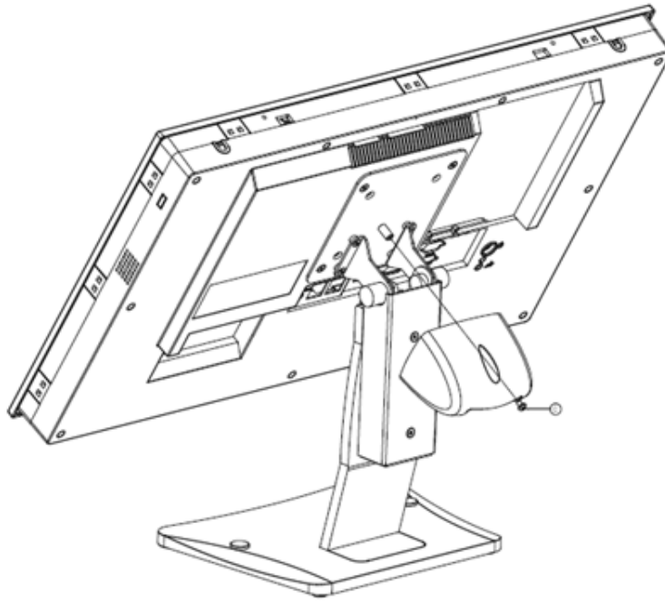
Securing the stand mount hinge cover
