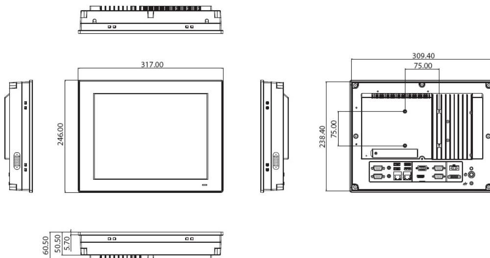
Figure 1.4 PPC-3120-RE9A Dimensions
