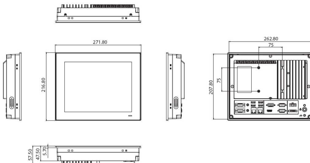
Figure 1.3 PPC-3100-RE9A Dimensions
